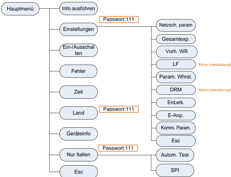
Fig. 7-1 LCD-Menübaum
